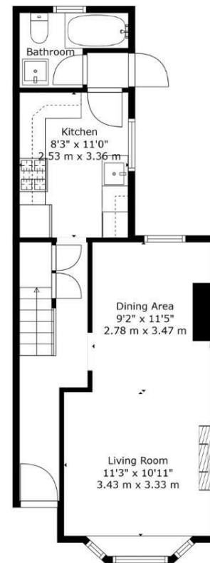
Floor 1
